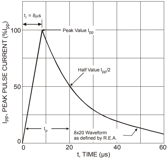
Figure 3 Pulse Waveform
